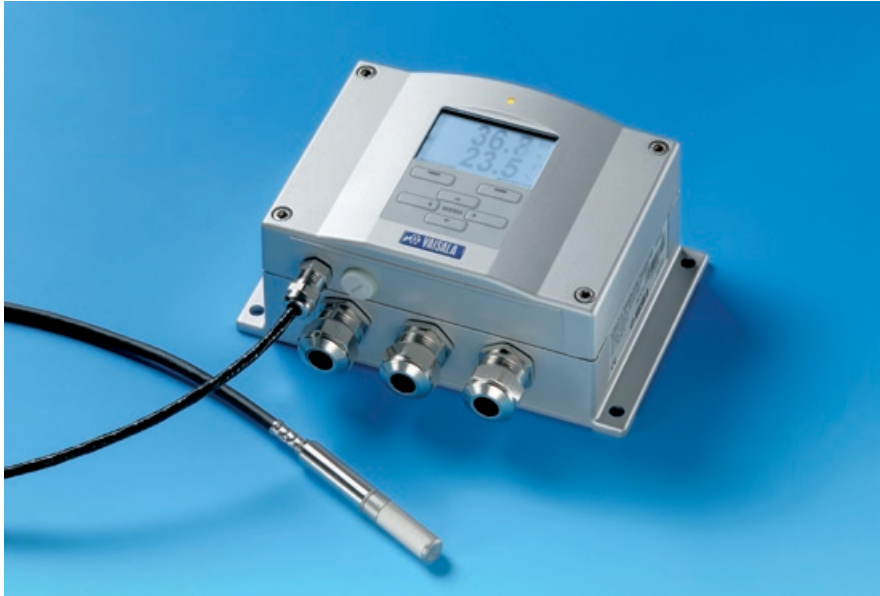
The HMT333 transmitter has a small probe for remote applications.
