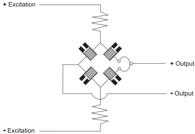
Figure 5-13. Load Cell
